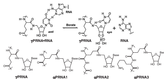
Chart 1. Structure of \gamma PRNA and \alpha PRNAs.
