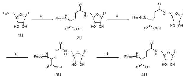
Scheme 1. Reagents: (a) N -Boc-L-Glu-OBzl, Bop reagent, HOBt, DIEA, DMF, 83%; (b) TFA; (c) Fmoc-OSu, DIEA, DMF, 90%; (d) H 2 , Pd/C, DMF/methanol, 96%.
