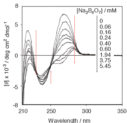
Figure 1. CD spectral changes of \alpha PRNA3 with increasing concentrations of \text{Na}_2\text{B}_4\text{O}_7 in phosphate buffer (0.033 M \text{KH}_2\text{PO}_4 –0.033 M \text{Na}_2\text{HPO}_3 , pH 7.2); [\alpha\text{PRNA3}] = 1.0 \times 10^{-4} M.
